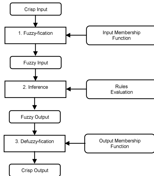
Fig.2. Fuzzy Logic
