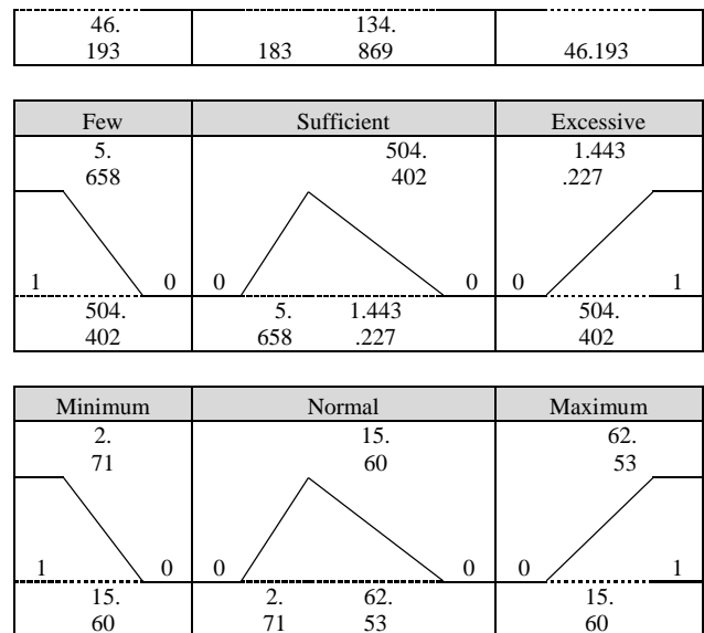
Fig.4. Curve Triangular
