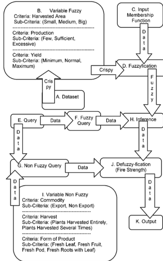
Fig.1. Framework
