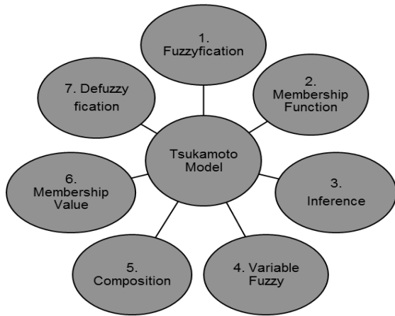
Fig.5. Tsukamoto Model
