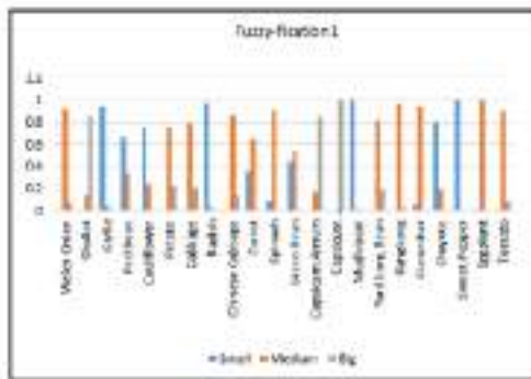
Fig.6. Graphic of Fuzzy-fication 1
